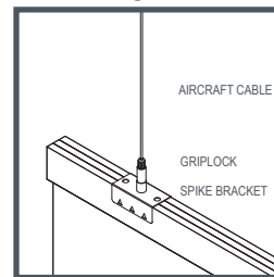
27mm Spike Bracket
